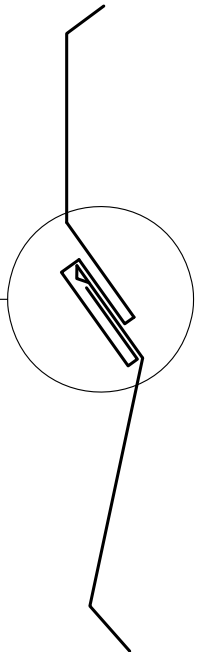
OPTIONAL JM 2 PIECE COUNTERFLASHING SURFACE VERSION (CFW2-500)
