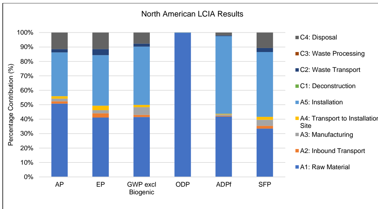
Figure 6: Contribution analysis of North American LCIA Results
