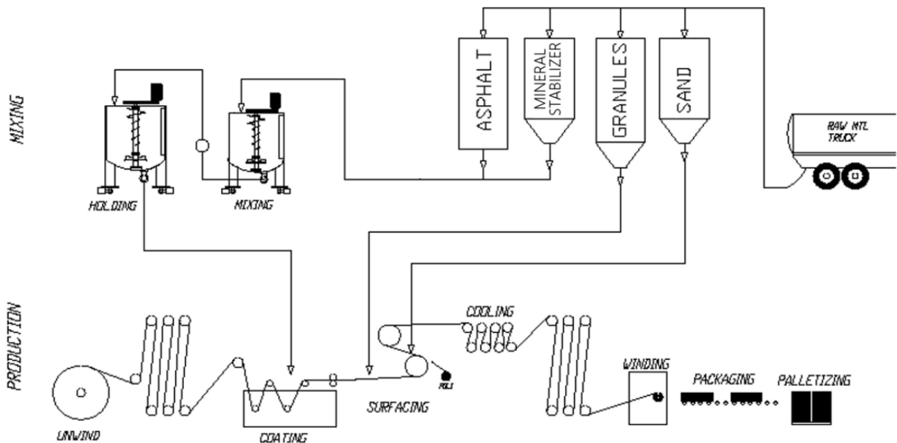
Figure 2: Mineral-surfaced cap sheet process diagram
