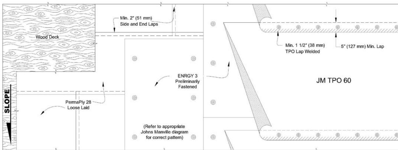
JM TPO 60 Mil Mechanically Fastened Membrane System Over ENRGY 3 ® Insulation and PermaPly ® 28 Base Sheet Loose Laid on a Wood Deck
