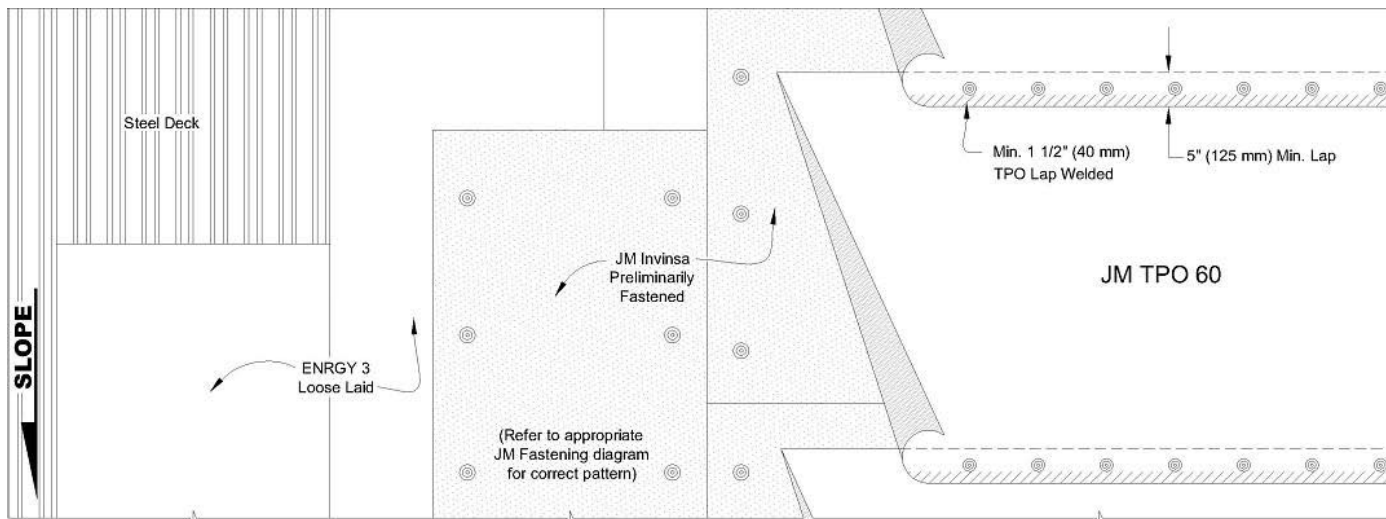
JM TPO 60 Mil Mechanically Fastened Membrane System Over ENRGY 3® Insulation and InvinSA™ Coverboard Fastened to a Steel Deck
