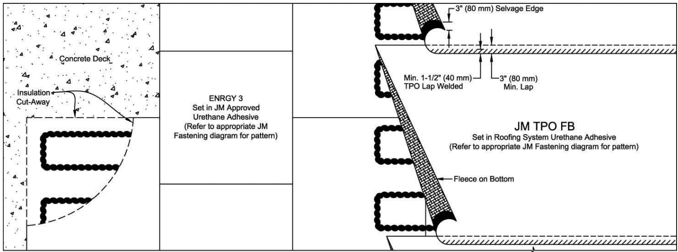
JM TPO FB 115 or 135 Fully Adhered Over ENRGY 3 Insulation Set in Adhesive
