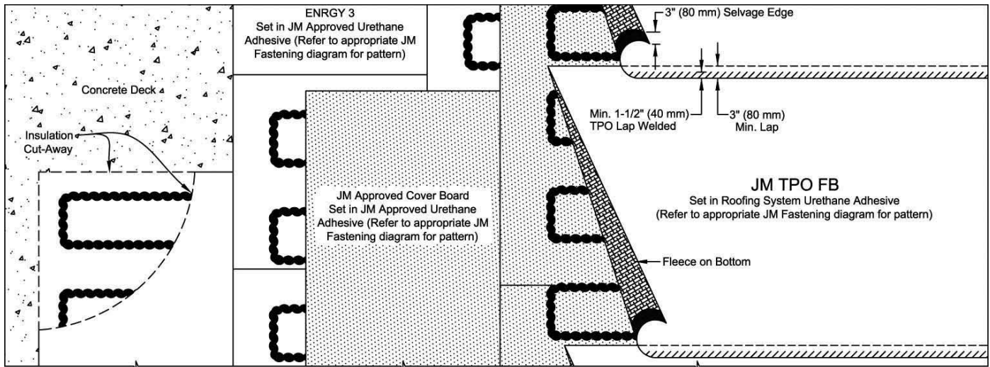
JM TPO FB 115 or 135 Fully Adhered Over JM Approved Cover Board and ENRGY 3 Insulation Set in Adhesive
