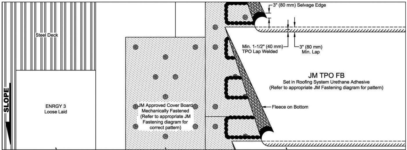
JM TPO FB 115 or 135 Fully Adhered Over ENRGY 3 Insulation and JM Approved Cover Board Fastened to a Steel Deck
