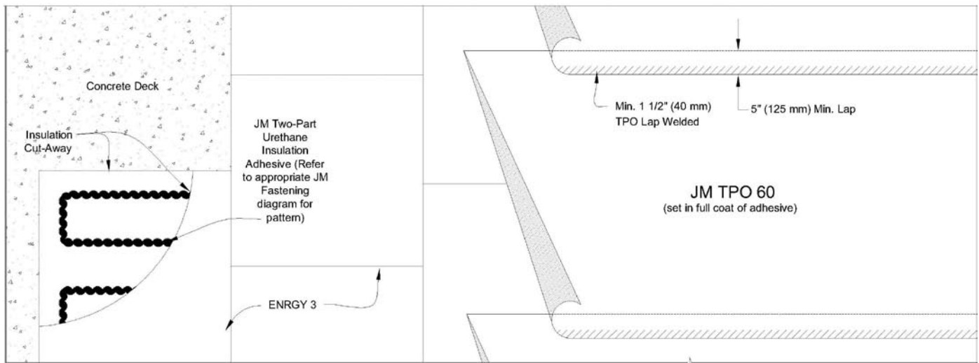
JM TPO 60 Mil Fully Adhered System Over ENRGY 3® Insulation Fastened to a Concrete Deck
