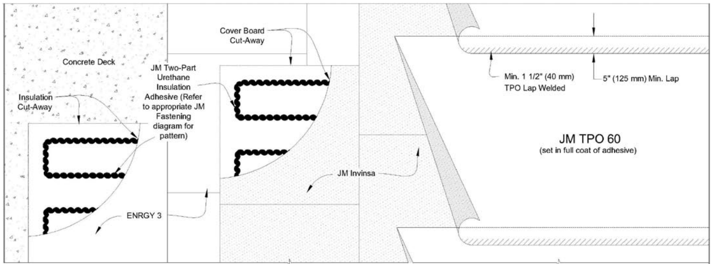
JM TPO 60 Mil Fully Adhered Membrane System Over ENRGY 3® Insulation and Invinsa™ Coverboard Fastened to a Concrete Deck
