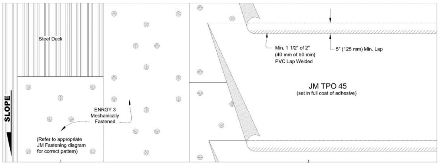
JM TPO 45 Mil Fully Adhered Membrane System Over ENRGY 3® Insulation Fastened to a Steel Deck
