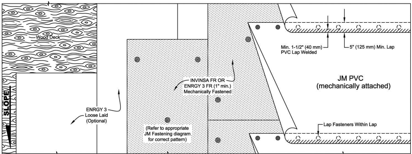
JM PVC 50, 60, 72 min, or 80 mil Mechanically Fastened Membrane System Over Invinsa® FR OR ENRGY 3® FR (1" min.) and ENRGY 3 Loose Laid (Optional)
