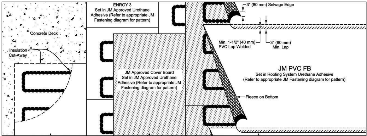
JM PVC Fleece-Backed 50 mil, 60 mil, 60 mil min, 72 mil min or 80 mil Fully Adhered Over JM Approved Cover Board and ENRGY 3 Insulation Set in Adhesive
