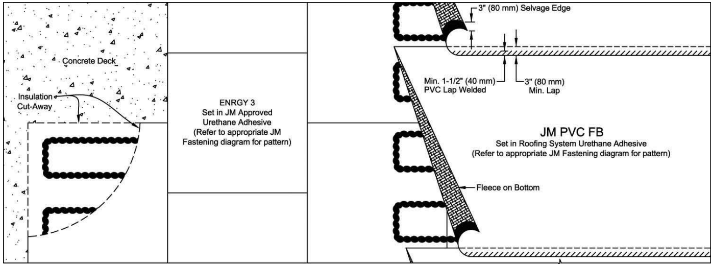
JM PVC Fleece-Backed 50 mil, 60 mil, 60 mil min, 72 mil min or 80 mil Fully Adhered Over ENRGY 3 Insulation Set in Adhesive
