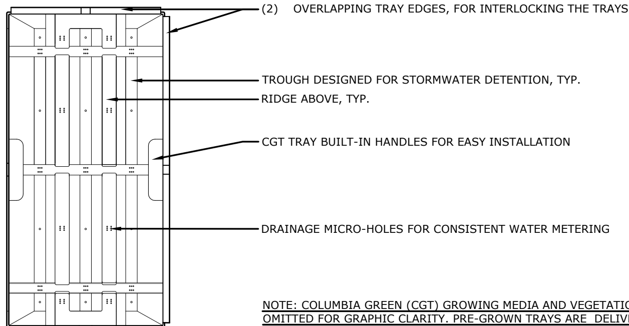
1'-0" L X 2'-0" W X 4.63" H TRAY PLAN
