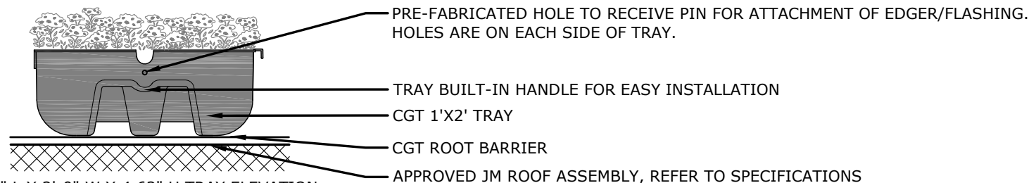
1'-0" L X 2'-0" W X 4.63" H TRAY ELEVATION
