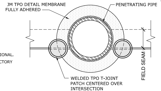
PLAN VIEW PENETRATION POCKET OVER FIELD SEAM
