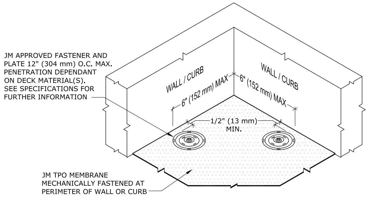
DECK ATTACHMENT
