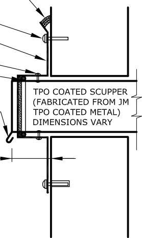
SCUPPER SECTION AT EXTERIOR WALL
