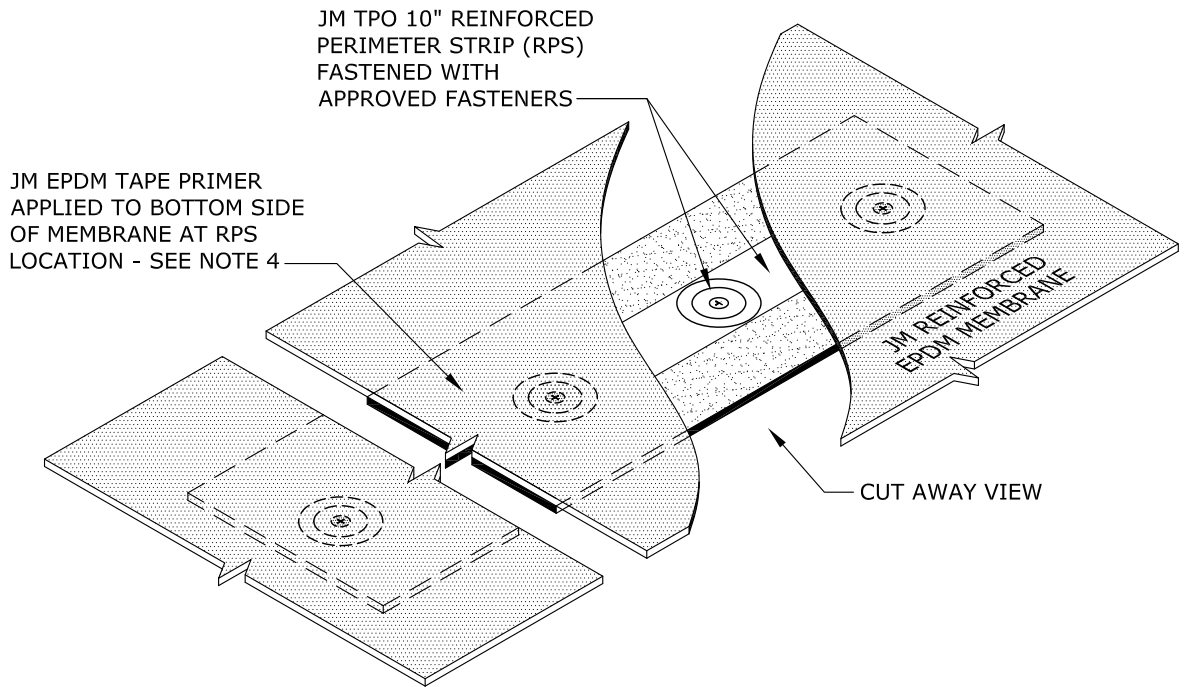
ISOMETRIC VIEW
