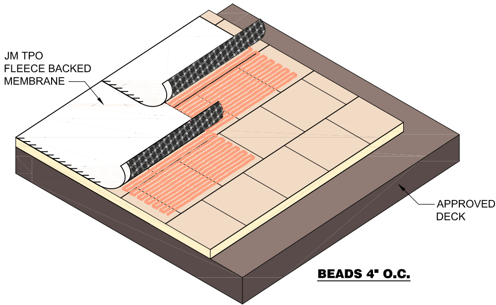
FIELD FASTENING
