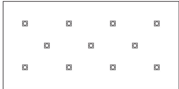
11 per 4x8 board with Adhered Non-Reinforced Membrane (EPDM)
