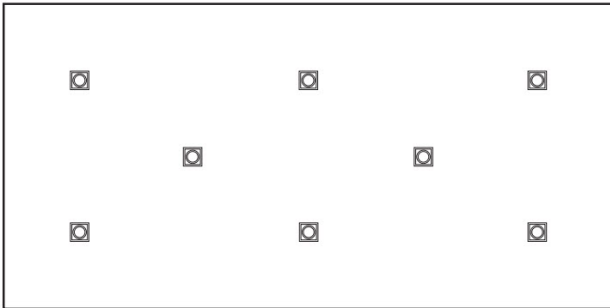
8 per 4x8 board with Adhered Reinforced Membrane (TPO, PVC, EPDM-R, Mod Bit)
