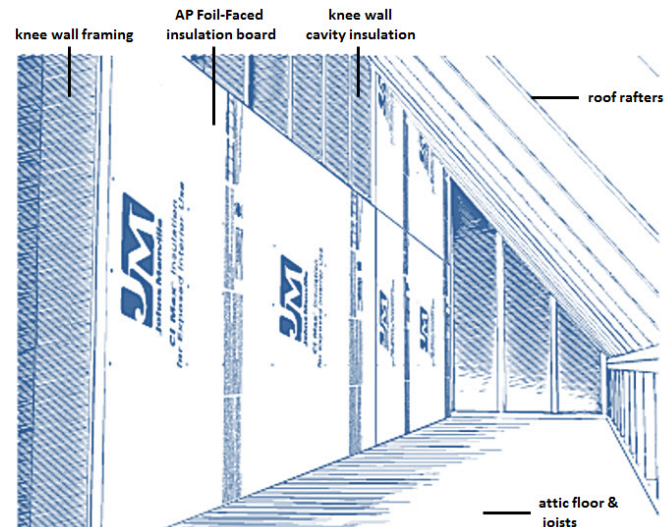
Figure 4. Knee Walls
