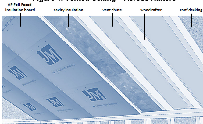
Figure 1. Vented Ceiling – Across Rafters
