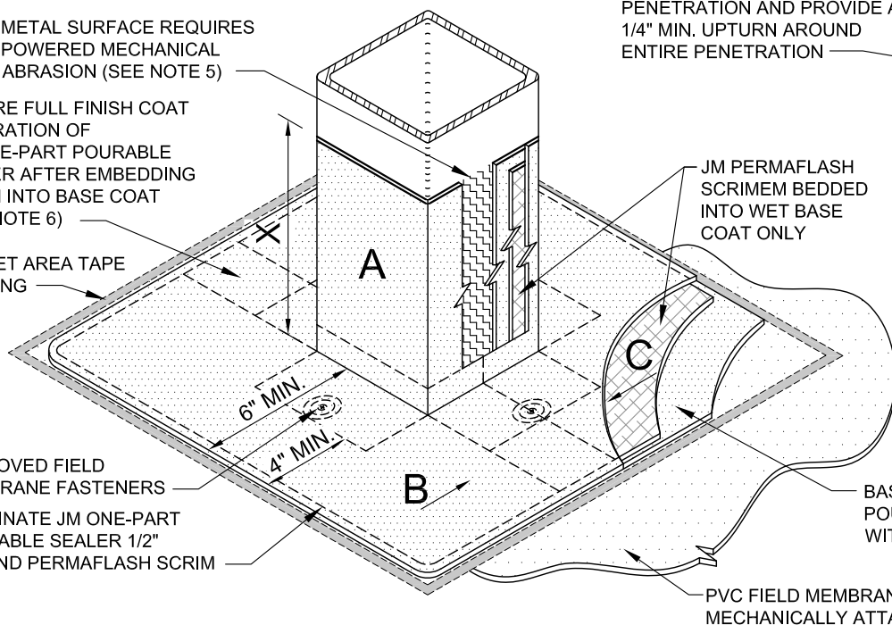
SCRIM HORIZONTAL VIEW STEPS B & C
