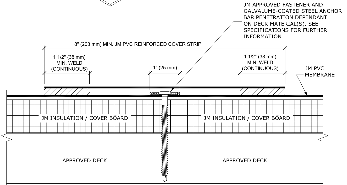
ISOMETRIC VIEW
