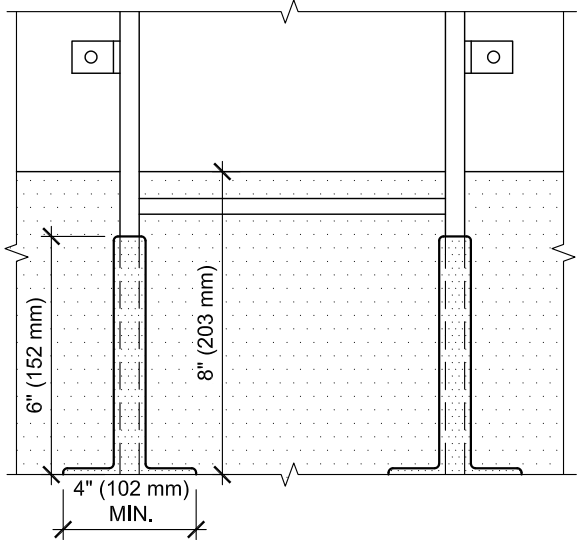
LADDER ELEVATION
